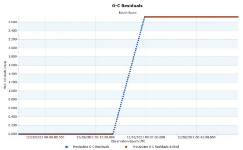
Figure 22. Observed Minus Computed MCC-1b Residuals of Tracking Data
