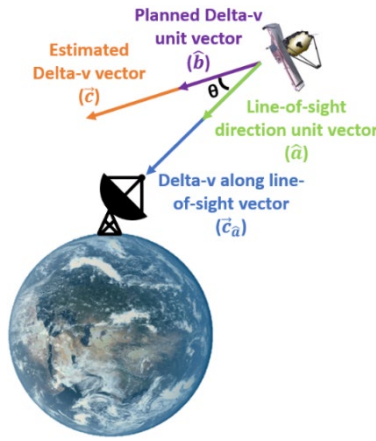
Figure 5. DVALOS (Delta-V Along Line-of-Sight) Algorithm Representation
