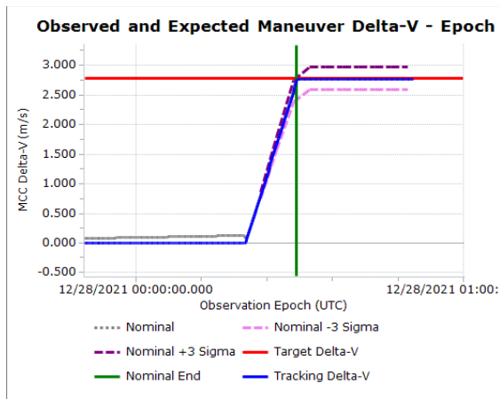
Figure 20. Observed and Expected MCC Delta-V versus Observed UTC Epoch
