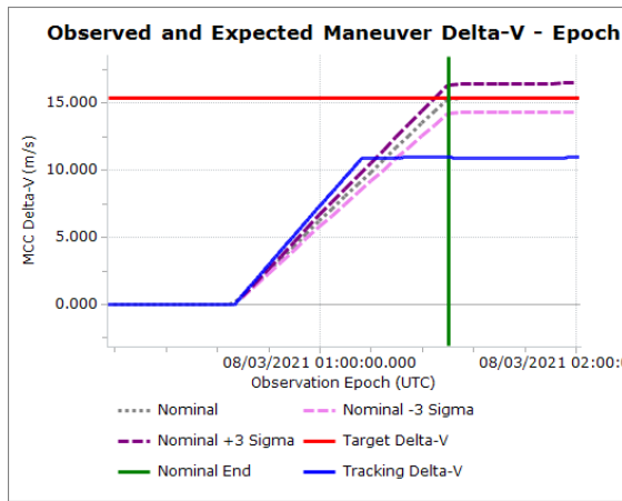
Figure 11. Delta-V for MCC-1a Overburn
