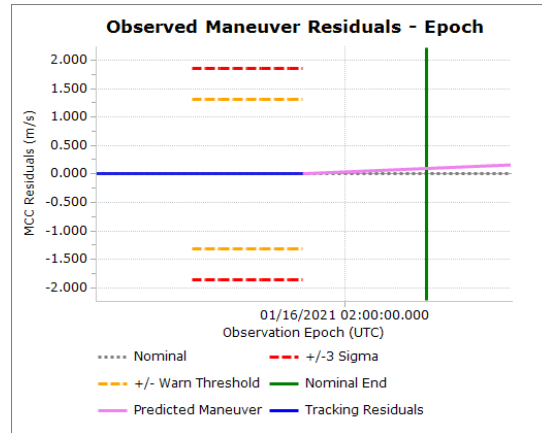
Figure 9. Mid-Maneuver Observed Residuals Nominal Case
