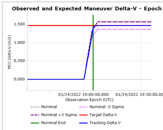
Figure 23. Observed and Expected MCC-2 Delta-V versus Observed UTC Epoch
