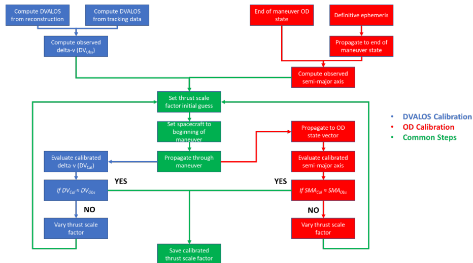
Figure 8. DVALOS & OD Calibration Methodologies
