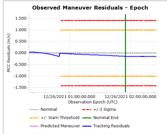
Figure 18. MCC Residuals versus Observed UTC Epoch
