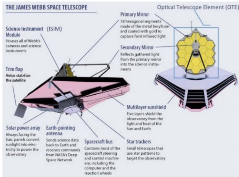
Figure 1. JWST Hardware Overview
