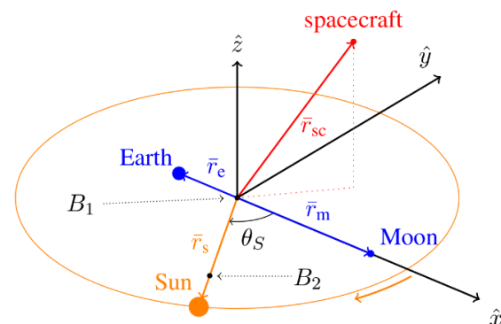
Figure 1. BCR4BP, Earth-Moon rotating frame
