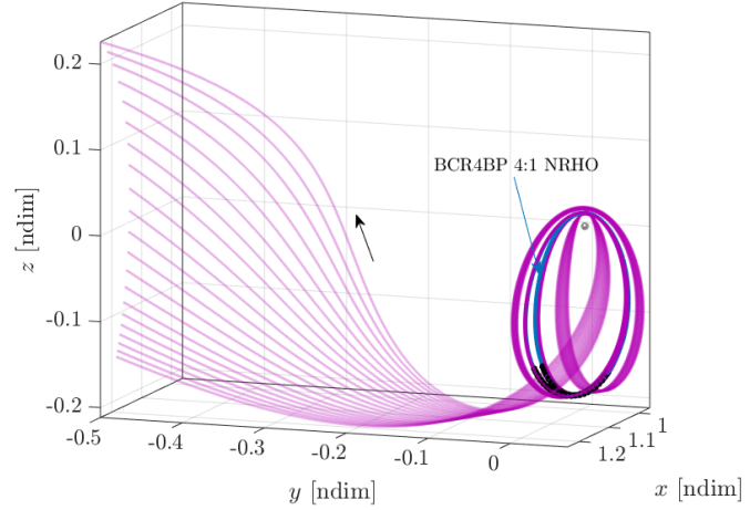
Figure 5. Representative unstable manifolds near apolune in the BCR4BP 4:1 NRHO.
