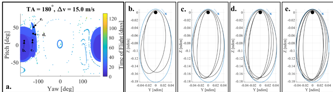
Figure 19. Differing multi-revolution transfers identified from variations in time to impact
