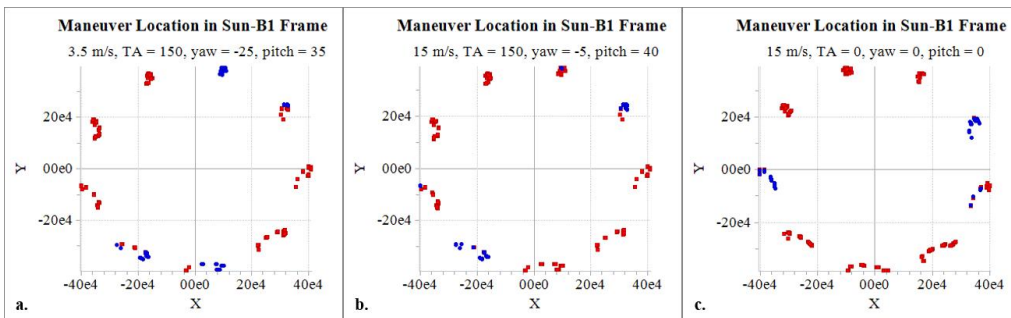
Figure 13. Maneuver orientations in the Sun- B_I frame in the ephemeris model.
